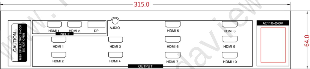
Rear panel
