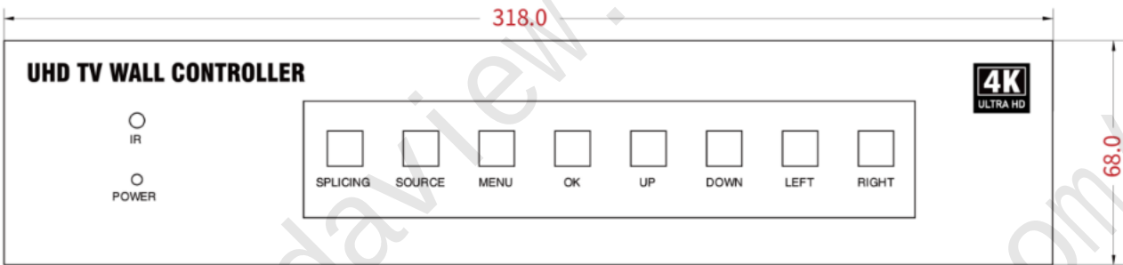
Front panel
